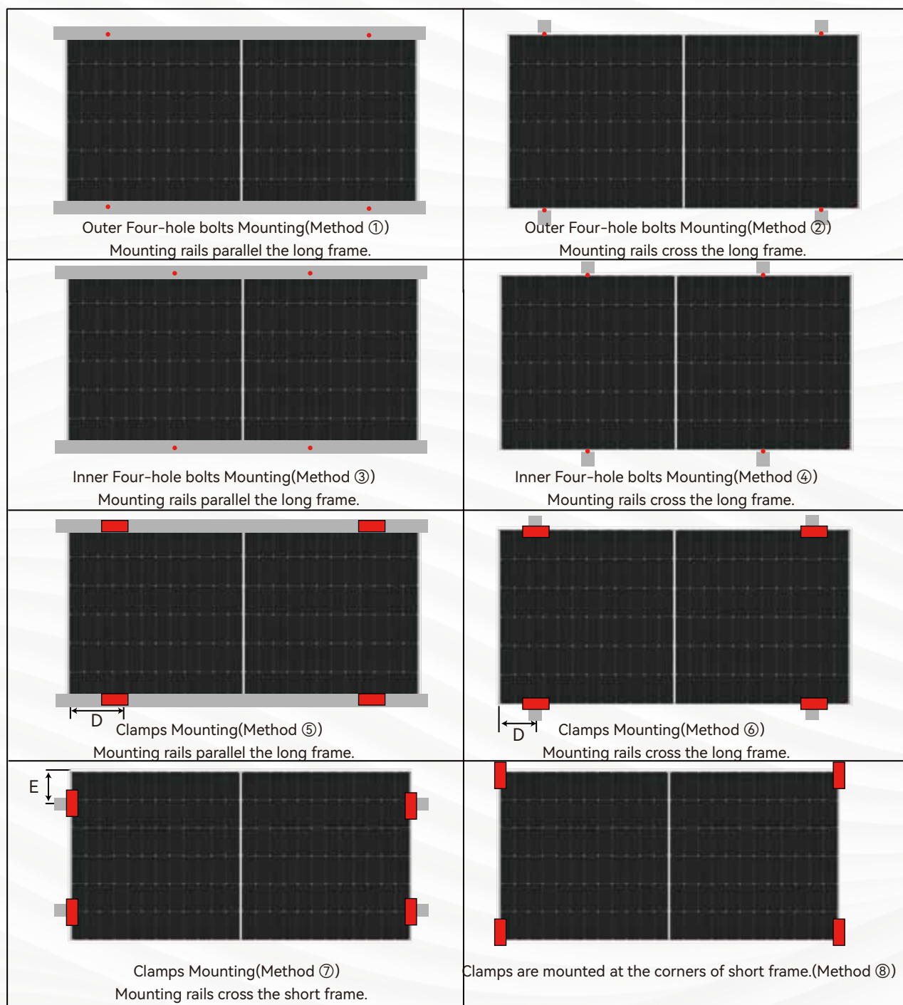
Figure 8 Bifacial Module Installation Position
